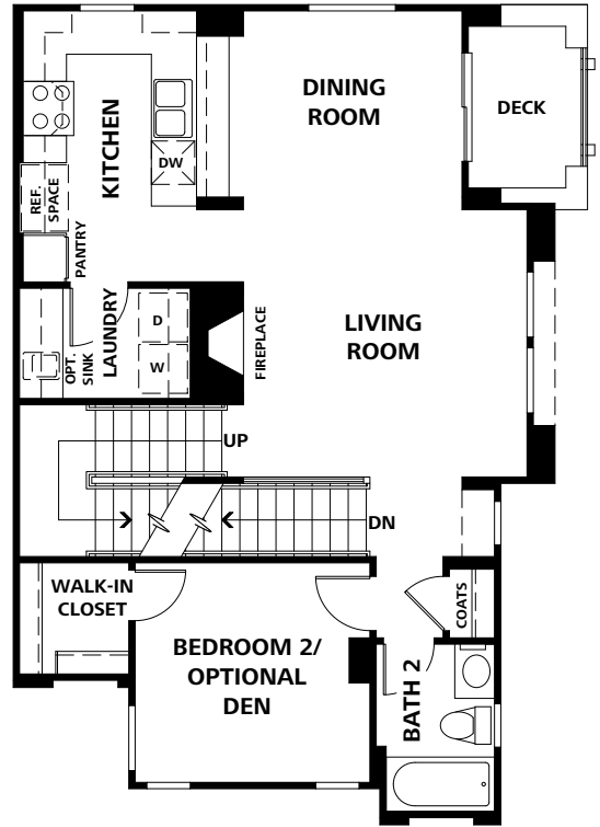
SECOND FLOOR
